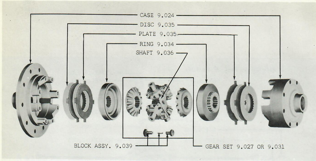
GROUP 9 - FIG. 2 - LOCKING DIFFERENTIAL CASE ASSEMBLY 20-80
