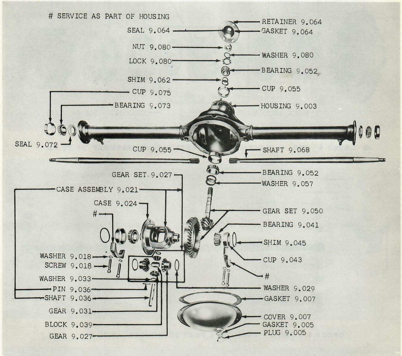
GROUP 9 - FIG. 1 - REAR AXLE 01-10-20-80
