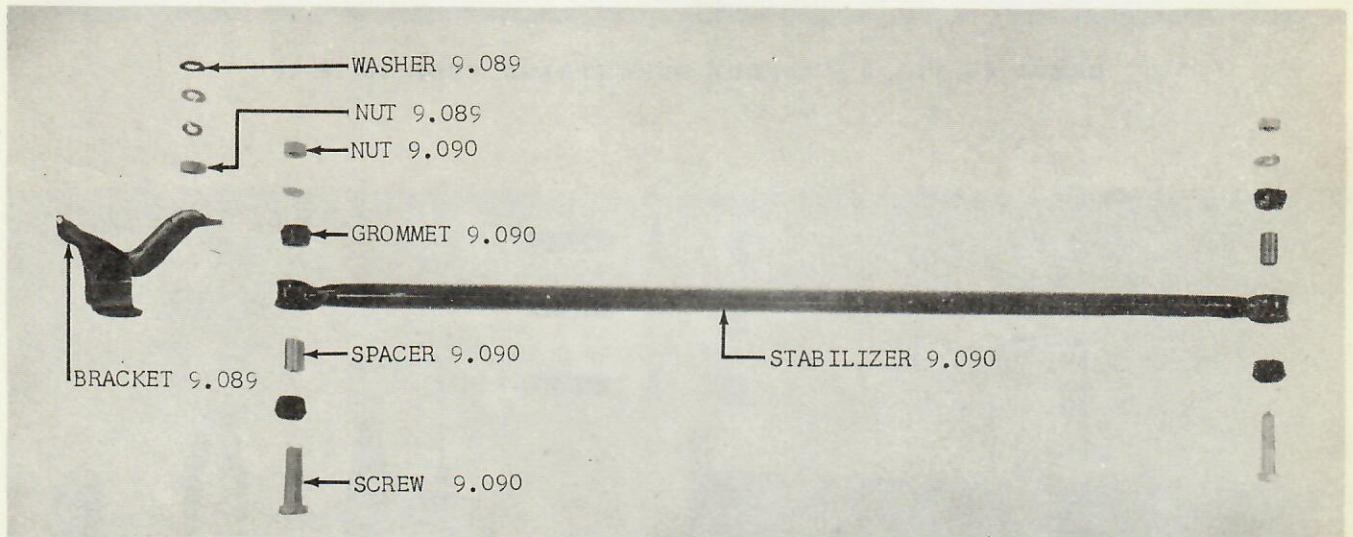
GROUP 9 - FIG. 3 - REAR AXLE SWAY STABILIZER 10-20-80
