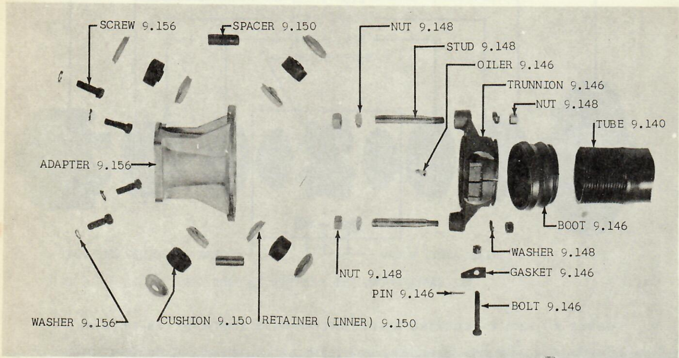
GROUP 9 - FIG. 5 - TORQUE TUBE (TRANS. END) 10-20-80
