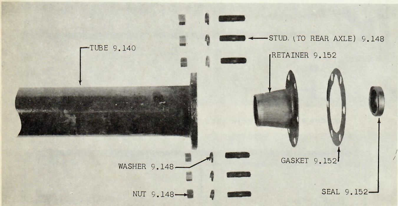
GROUP 9 - FIG. 6 - TORQUE TUBE (AXLE END) 10-20-80
